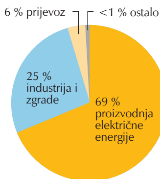
Slika 2 – \text{SO}_2 koji nastaje ljudskim djelovanjem (izvor: https://www.e-inst.com/training/combustion/sulfur-compound-emissions/ )
