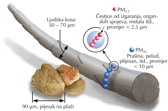
Slika 3 – Usporedba veličine PM čestica (izvor: https://www.epa.gov/pm-pollution/particulate-matter-pm-basics )
