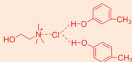
DES-7
